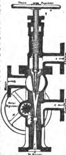
FIG. 56.—Giffard's Injector.
