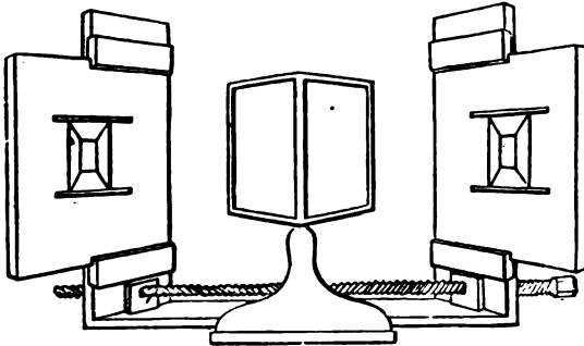
FIG. 2.—Wheatstone's Reflecting Stereoscope.
