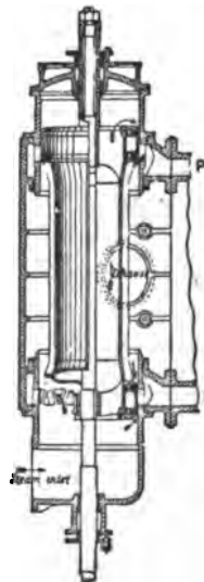
Fig. 86.—Piston Slide-Valve.
