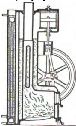
Fig. 133.—Davey Motor.
