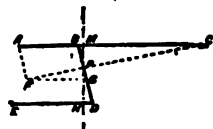
FIG. 119.—Watt's Parallel Motion.
