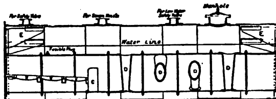
FIG. 39.—Cornish Boiler: longitudinal section.
