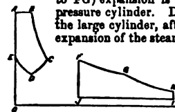
FIG. 30.—Compound Diagrams: Receiver type.
