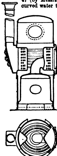
FIG. 49.—Vertical Boiler: Tubular Form.
