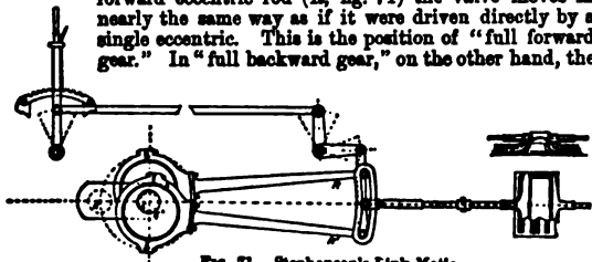
Fig. 71.—Stephenson's Link-Motion
