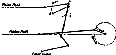
Fig. 78.—Diagram of Joy's Valve-Gear.
