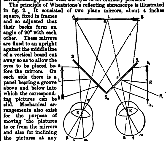
FIG. 2.—Diagram of Wheatstone's Reflecting Stereoscope. K, K', right and left eyes; S, S', mirrors; L, R, panels for holding pictures; a, b, pictures on left side; a', b', pictures on right side; a, b, A and a', b' are corresponding points on retinas; A, L, object as seen in relief in mirrors; b, seen by left eye in position B, and image on retina at \beta ; L seen at L, R, and retinal image at \lambda ; a seen at A, and retinal image at \alpha ; a' seen at A, and retinal image at \alpha' ; B seen at B, and retinal image at \beta ; U seen at B, and retinal image at \beta .—Landolt and Stirling's Physiology .
