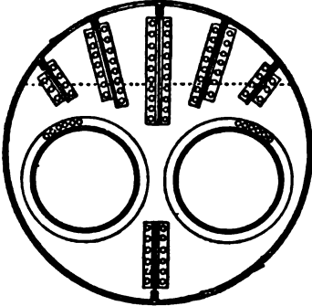
FIG. 41.—Lancashire Boiler: Transverse Section. sloping down towards the back, where they terminate at the "bridge" of fire-brick (C, fig. 39). Beyond the bridge the flue is crossed by a number of tapered "Galloway" tubes D, E, which increase the heating surface, promote circulation of the water, and stiffen the flue. The end plates are strengthened by gusset stays
