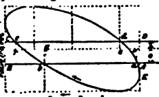
Fig. 65.—Oval Diagram of Slide-Valve Motion.
