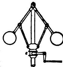
FIG. 90.—Watt's Governor.
