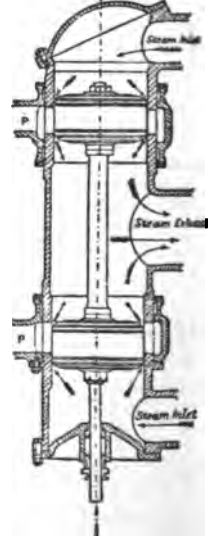
Fig. 87.—Piston Slide-Valve.
