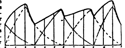
Fig. 116.—Crank-Effort Diagram for Two Cranks.
