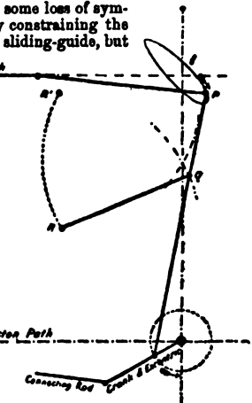
Fig. 77.—Bremme's or Marshall's Valve-Gear.
