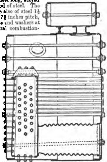
Fig. 55.—Single-Ended Marine Boiler.
