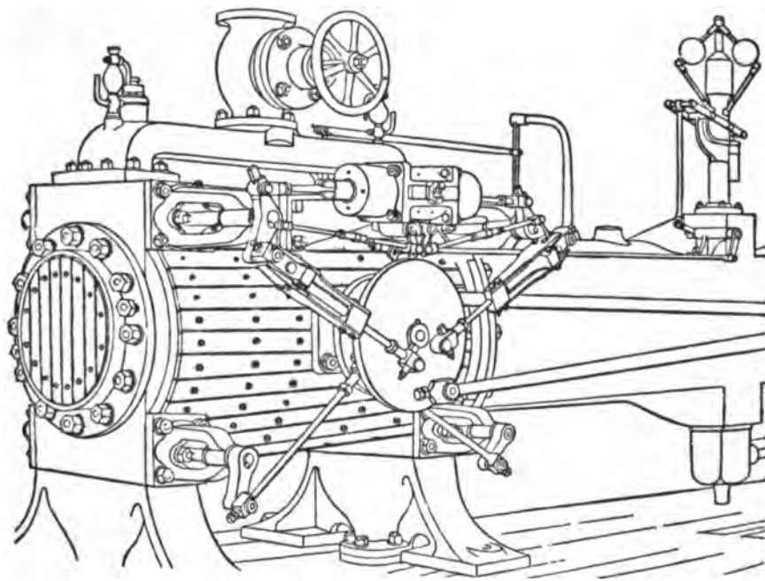
FIG. 101.—Corliss Engine, with Spencer Ingalls Trip-Gear.
