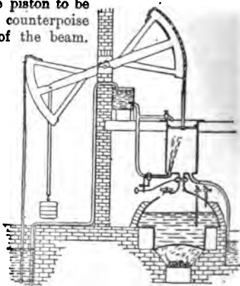
FIG. 4.—Newcomen's Atmospheric Engine, 1705.
