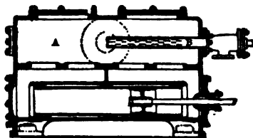
FIG. 126. Condenser and Air-Pump.
