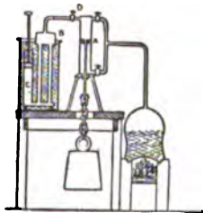
FIG. 5.—Watt's Experimental Apparatus.
