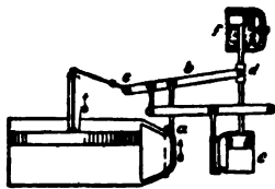
FIG. 107.—Davey's Differential Valve-Gear.
