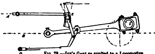
Fig. 79.—Joy's Gear as applied to a Locomotive.
