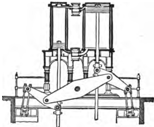
FIG. 130.—Vertical Non-Rotative Pumping Engine.
