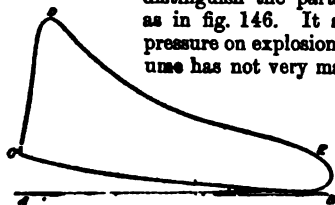
FIG. 147.—Otto Engine Diagram.
