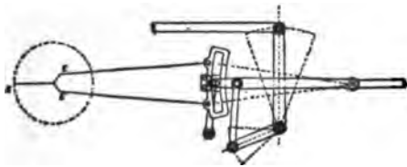
Fig. 72.—Gooch's Link-Motion.
