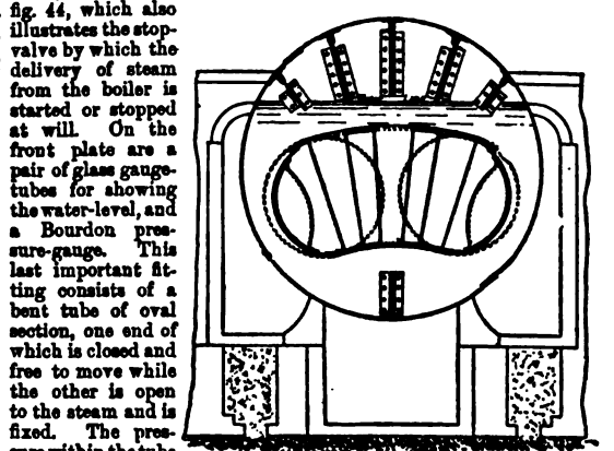
FIG. 46.—Galloway Boiler: Section beyond the Bridge.
