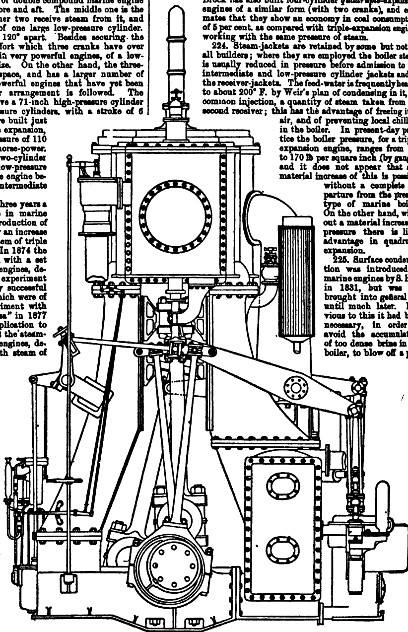
FIG. 125.—End Elevation of Marine Engine.
