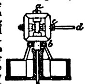
Fig. 106.—Siemens's Governor.
