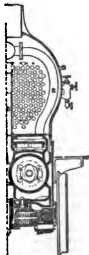
FIG. 138.—Inside-Cylinder Locomotive.
