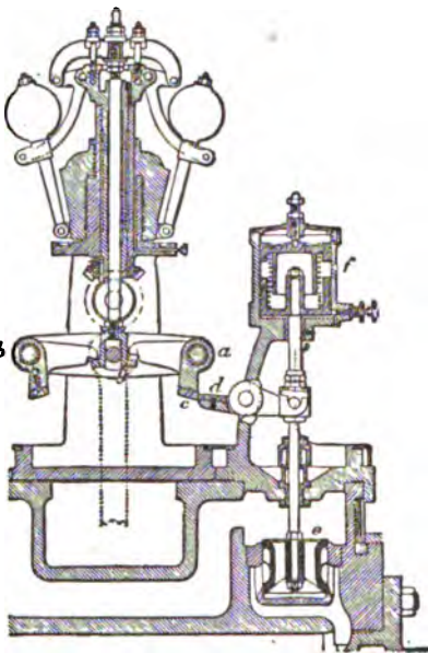
Fig. 103.—Proell's Automatic Expansion Gear.
