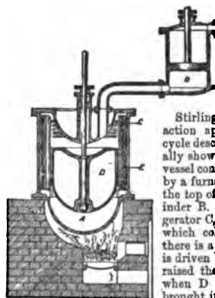
FIG. 141.—Stirling's Air-Engine.
