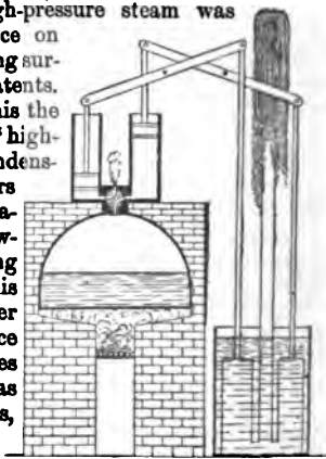
FIG. 8.—Leupold's Non-Condensing Engine, 1725.
