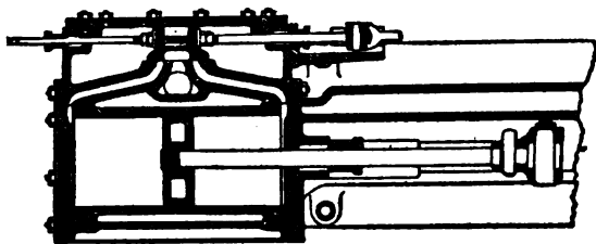
FIG. 124.—Horizontal Section through Cylinder and Valve-Chest.
