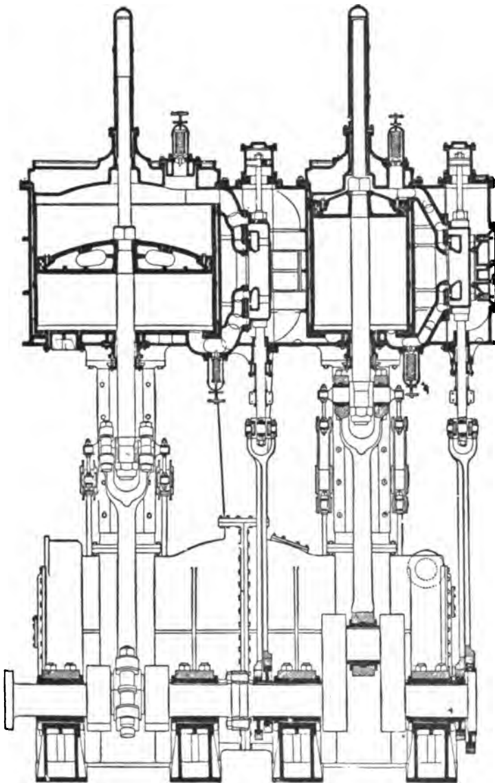
FIG. 134.—Longitudinal Section of Marine Engine.
