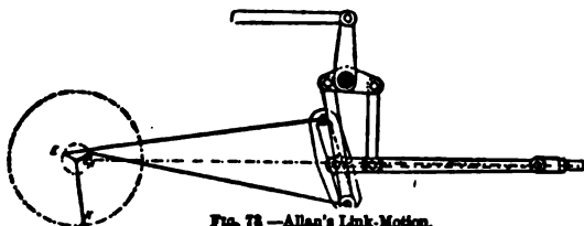
Fig. 73.—Allan's Link-Motion.
