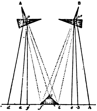
FIG. 4.—Diagram of the Refracting Stereoscope.
