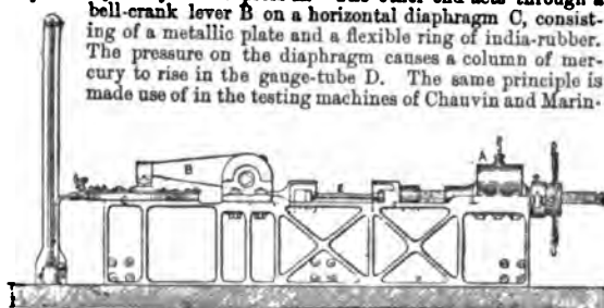
Fig. 9.—Thomasset's Testing Machine.
