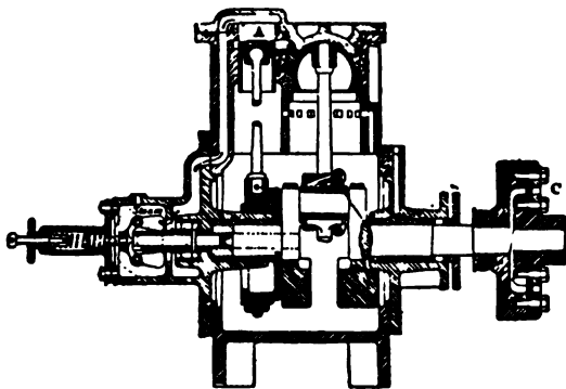
FIG. 128.—Brotherhood's Three-Cylinder Engine: longitudinal section.
