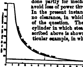
FIG. 18.—Ideal Indicator Diagram for Steam used expansively.
