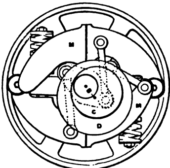
FIG. 100.—Governor of Armstrong & Sims Engine.
