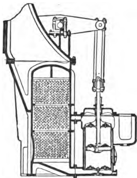
FIG. 187.—Section through Condenser and Air-Pump.
