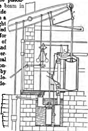
FIG. 7.—Watt's Double-Acting Engine, 1782.
