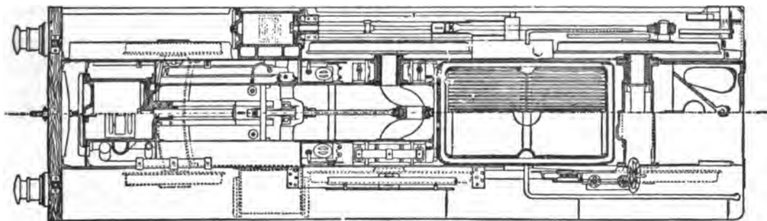
FIG. 140.—Webb's Compound Locomotive.
