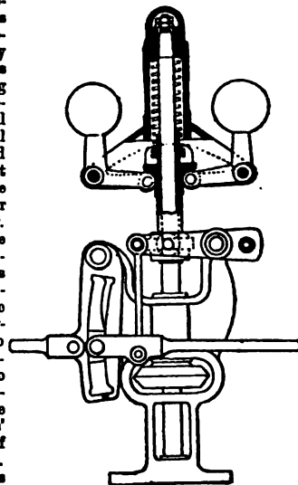
FIG. 99.—Hartnoll's Governor.
