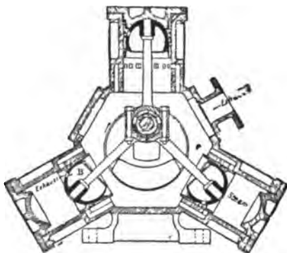
FIG. 129.—Brotherhood's Three-Cylinder Engine: transverse section.
