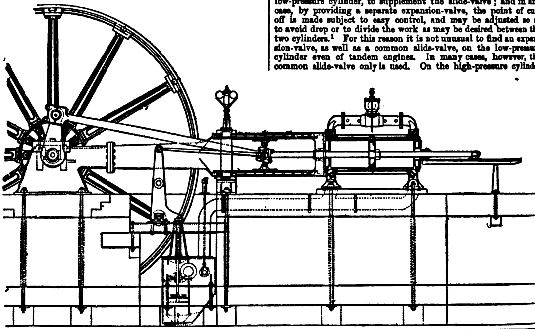
FIG. 127.—Horizontal Corliss Condensing Engine.
