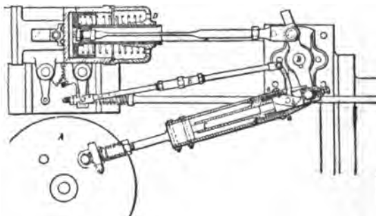
FIG. 102.—Corliss Valve-Gear, Spencer Ingalls form.
