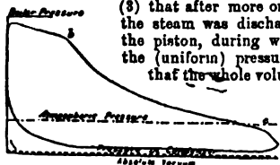
FIG. 18.—Actual Indicator Diagram from a Condensing Steam-Engine.
