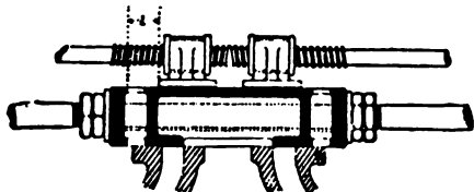
Fig. 83.—Expansion-Valve on back of Main Slide-Valve.
