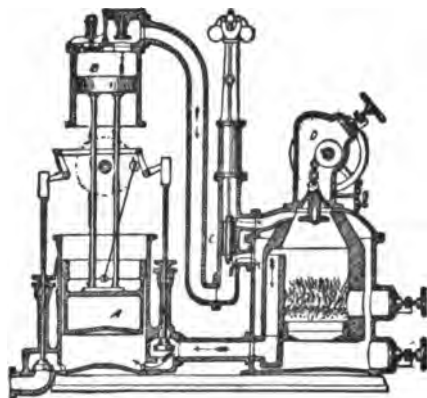
FIG. 142.—Bucket Engine.
