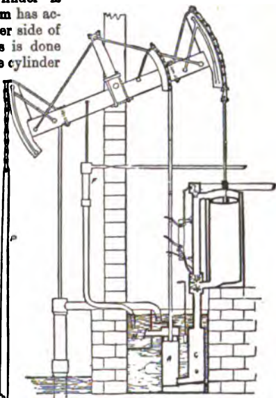
FIG. 6.—Watt's Single-Acting Engine, 1769.
