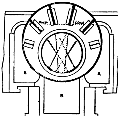
FIG. 40.—Cornish Boiler: transverse section, showing flues.
