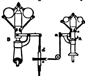
Fig. 104.—Knowles's Supplementary Governor.
