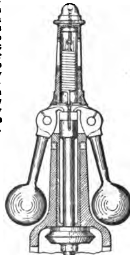
FIG. 92.—Spring Governor (Tangye).
