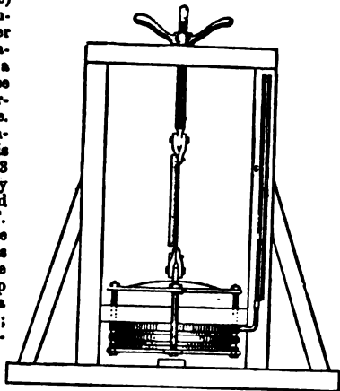
Fig. 8.—Hydraulic Machine for Testing Wire.
