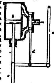
Fig. 105.—Differential Gear for Relay Governor.
